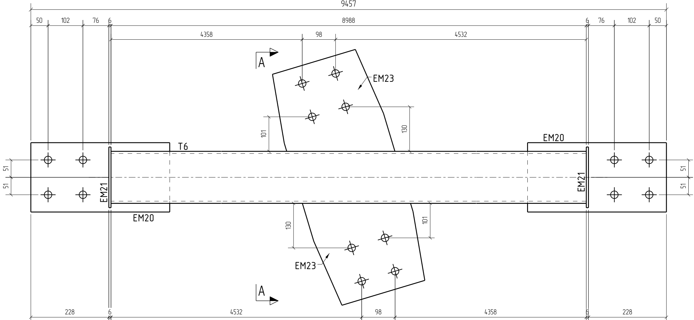
VISTA FRONTAL ESC: 1:6.5
